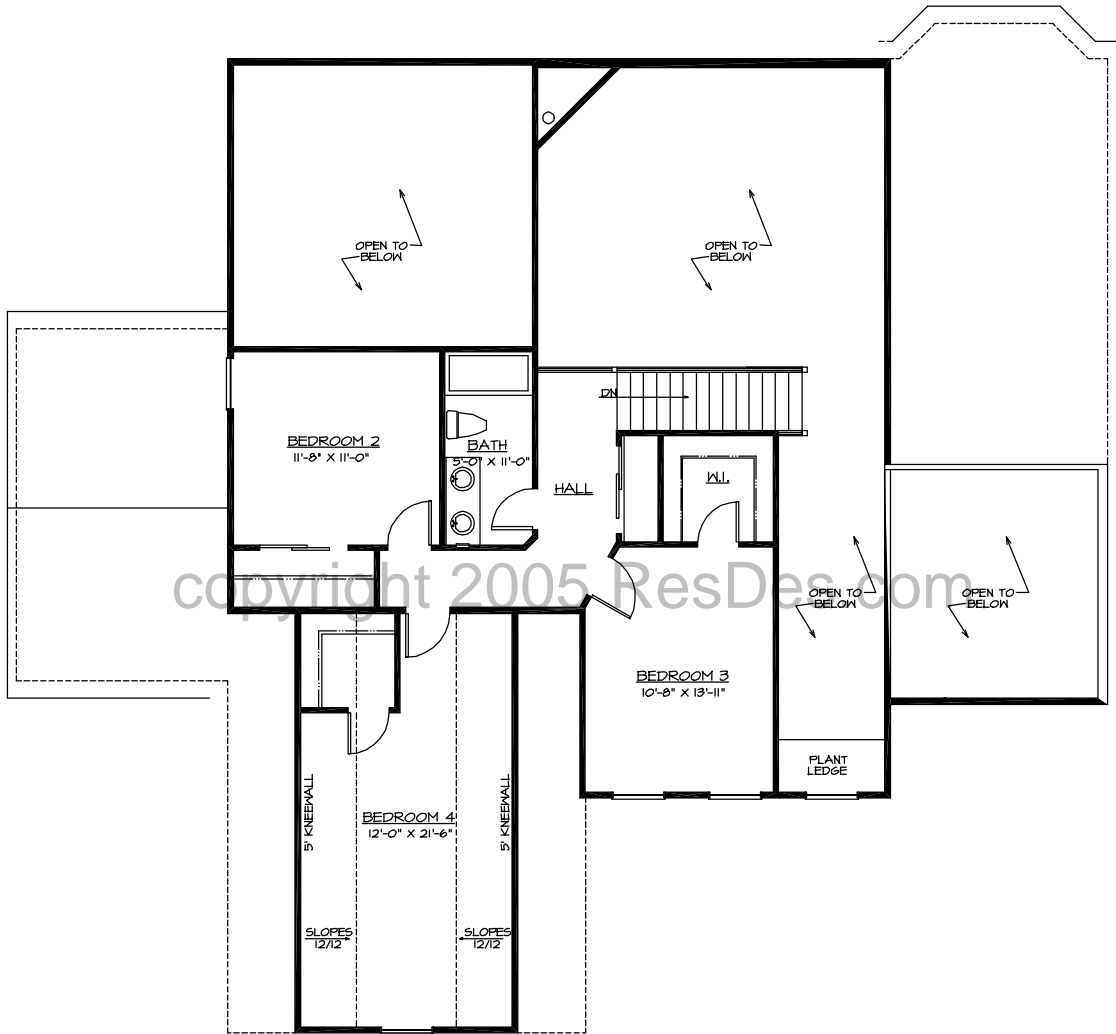
Second Floor
